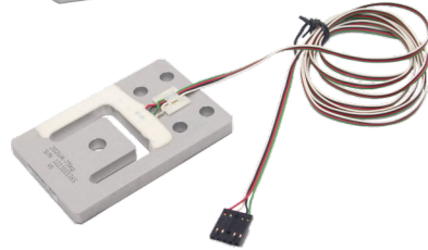
202UA-02: with Ribbon Cable & Connector
