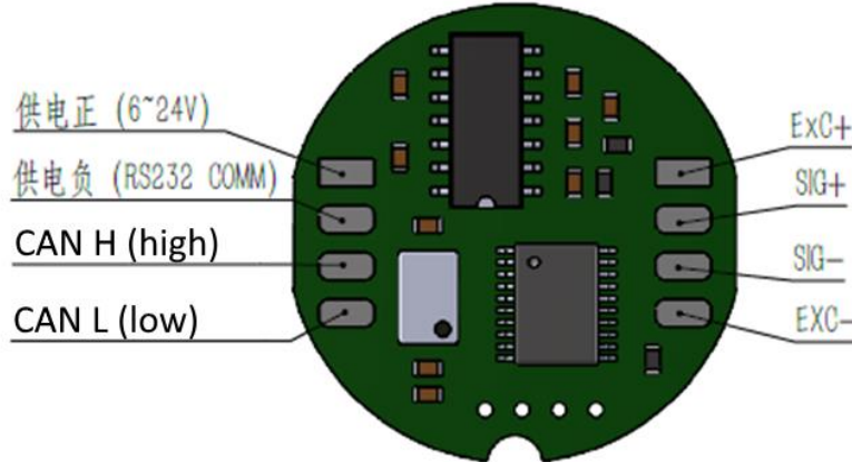
Figure 2-1: Connection Diagram for DGB-DC2508A
