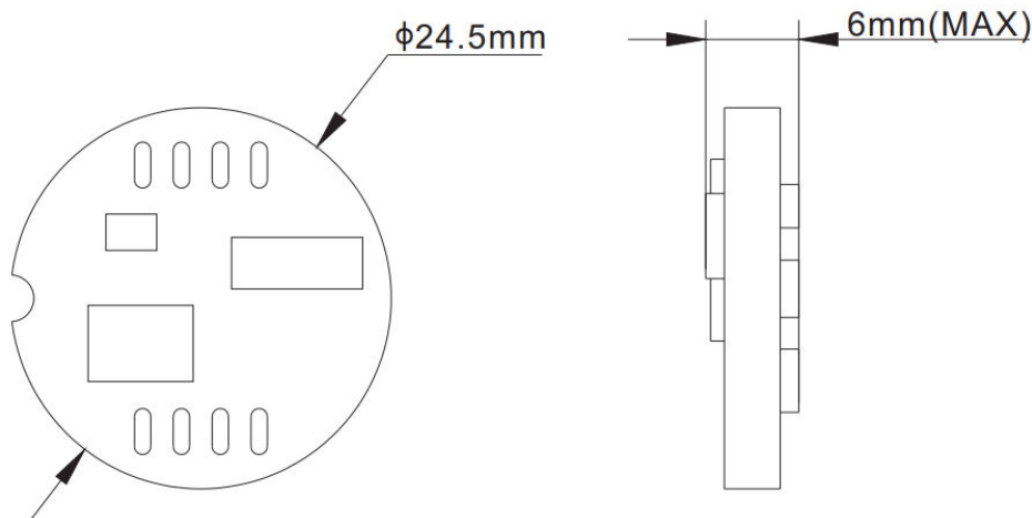
Figure 8-1: Chip Dimensions
