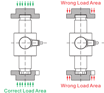
Installation diagram: Correct Load Area
