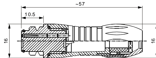
Female cable connector, cable outlet 4-6mm Contacts 3,5,8
