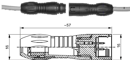
Male cable connector, cable outlet 4-6mm Contacts 3,5,8
