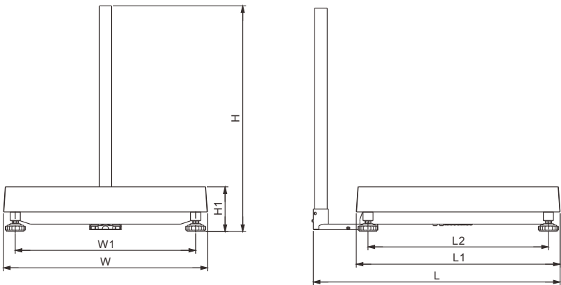
DIMENSIONS(mm)
